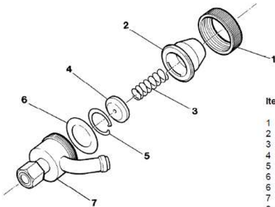
Fig. 11 – Diaphragm Check Valve
