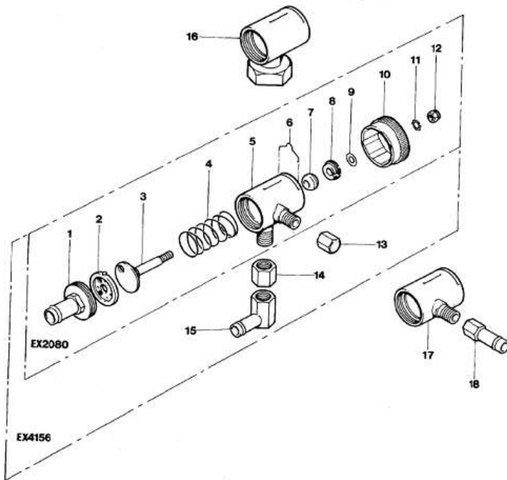
Fig. 10 – Variable Restrictor Units and Optional Adaptors
